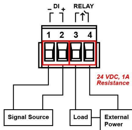
Figure 2.11 - Wiring the DI and Relay Alarm Contact
